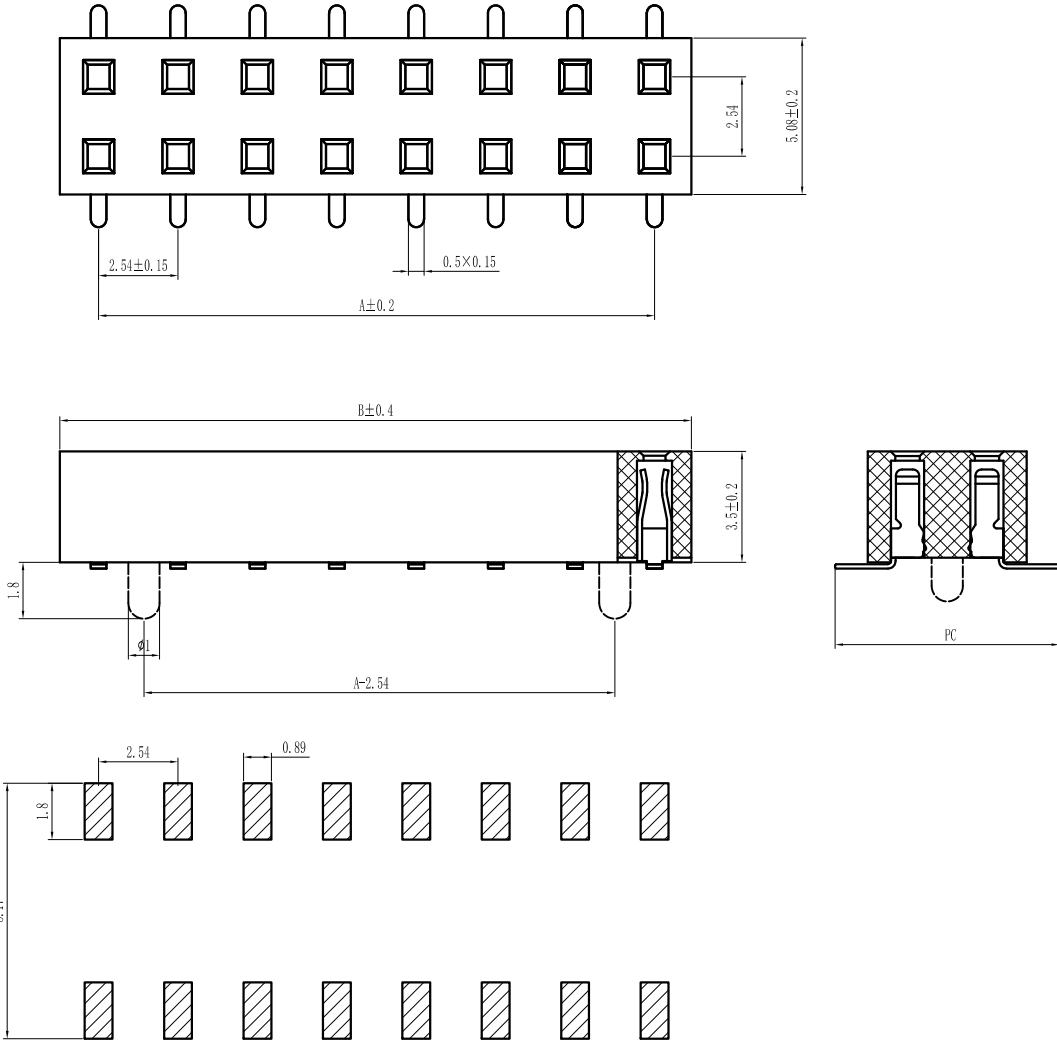
PCB LAYOUT
