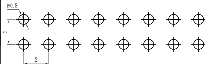
PCB LAYOUT
