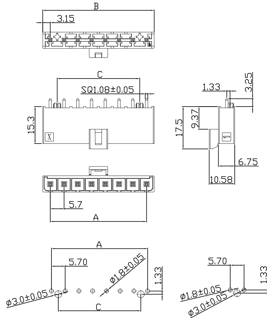
PCB board layout
