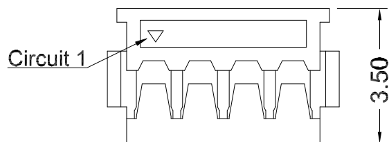
2~5Pin Shape
