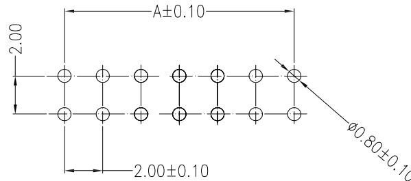
SUGGESTED PCB LAYOUT (COMPONENT SIDE)
