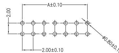
SUGGESTED PCB LAYOUT (COMPONENT SIDE)
