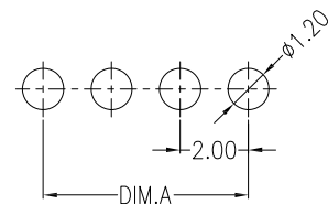
SUGGESTED PCB LAYOUT
