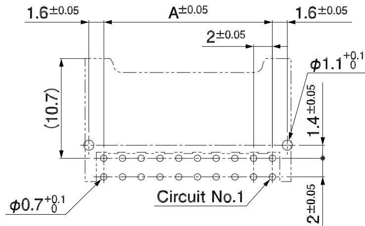
PCB LAYOUT
