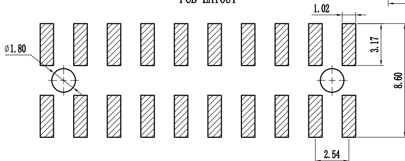
PCB LAYOUT
