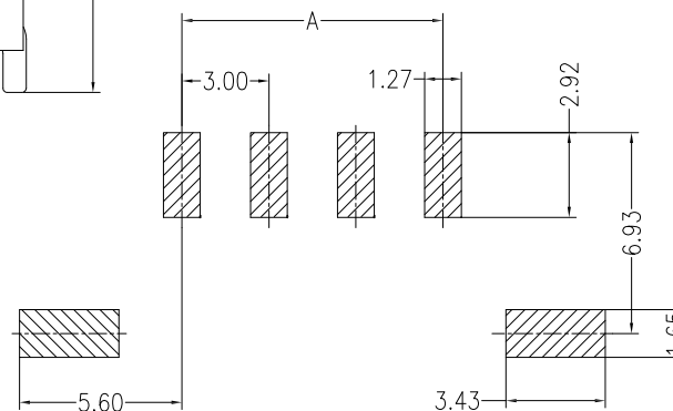
PCB LAYOUT(Tolerance: \pm 0.05 )
