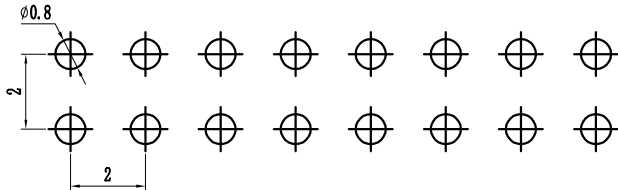
PCB LAYOUT
