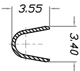
SECTION Z-Z CONDUCTOR CRIMP 14/16 AWG
