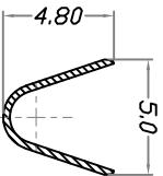
SECTION Z-Z CONDUCTOR CRIMP 12 AWG
