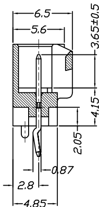
SECT. X-X
